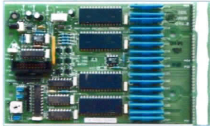
Figure 21-3 Small Diode Array PCB
