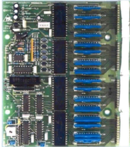
Figure 21-2 Large Diode Array PCB
