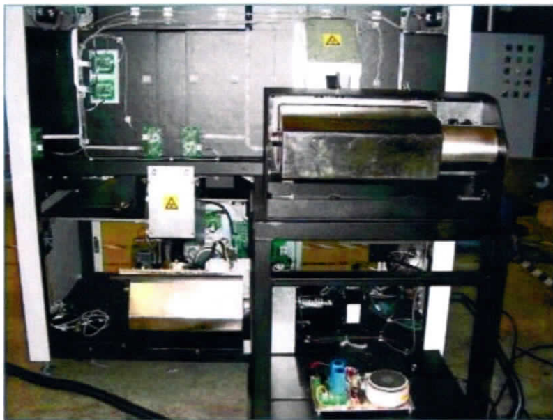
Figure 17-1: Vertical Generator (left) and Horizontal Generator (right)
